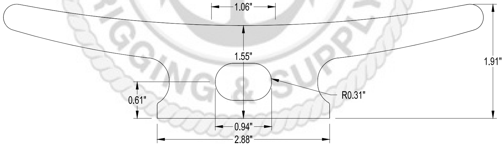
SIDE VIEW
