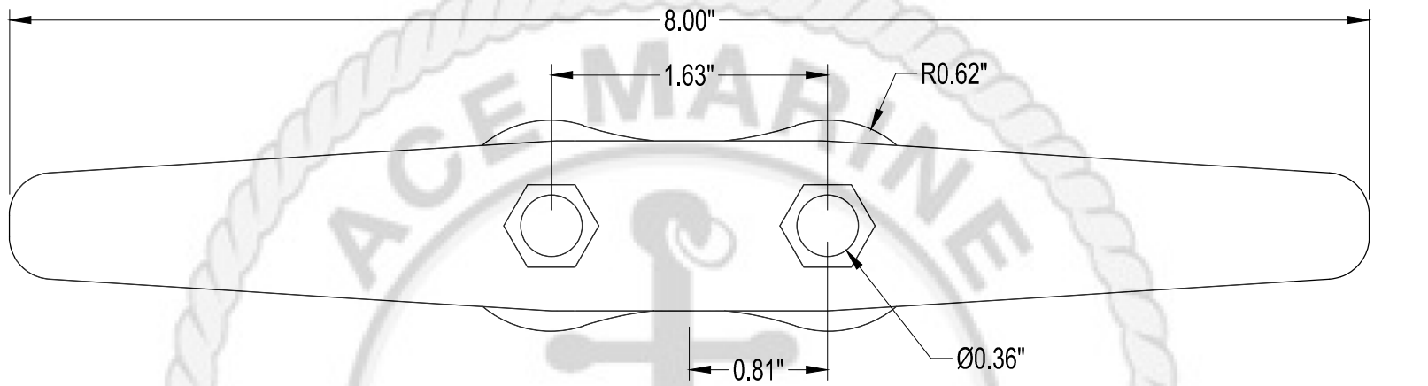
TOP VIEW
