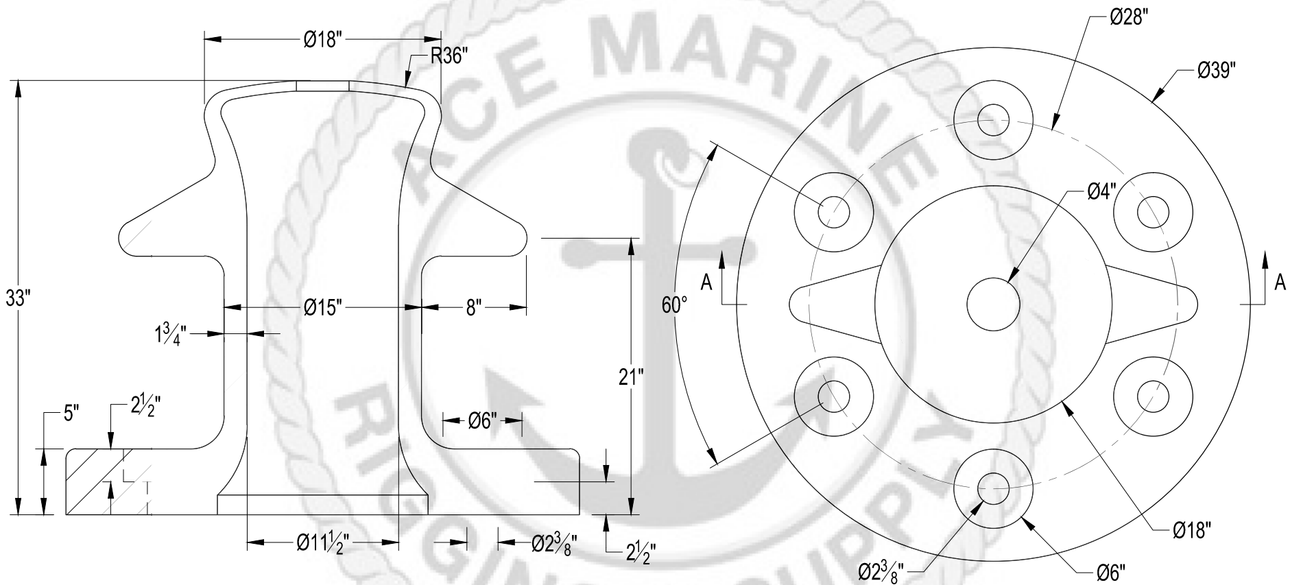
TOP VIEW
